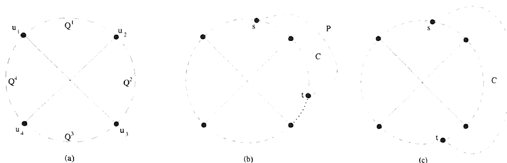
FIG. 6. Dotted and dashed curves indicate internally node disjoint paths; dashed curves have positive length, whereas dotted curves may have length zero. In (a), dashed curves have an even number of edges.
