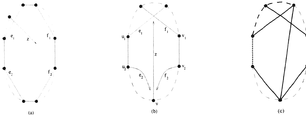
FIG. 10. Dotted and dashed curves indicate internally node disjoint even paths; dashed curves have positive length, whereas dotted curves may have length zero. The closed curve on the outside is the rim. The bold edges and curves in (c) form a test.
