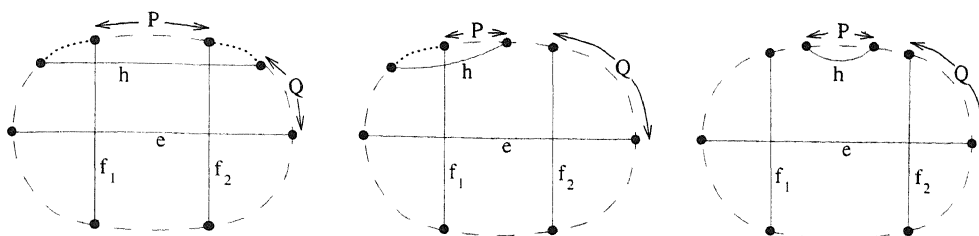
FIG. 8. Dotted and dashed curves indicate internally node disjoint even paths; dashed curves have positive length, whereas dotted curves may have length zero. The closed curve on the outside is the rim.
