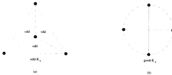
FIG. 1. Dashed curves indicate internally node disjoint paths of positive length, which in (b) all have even length.
